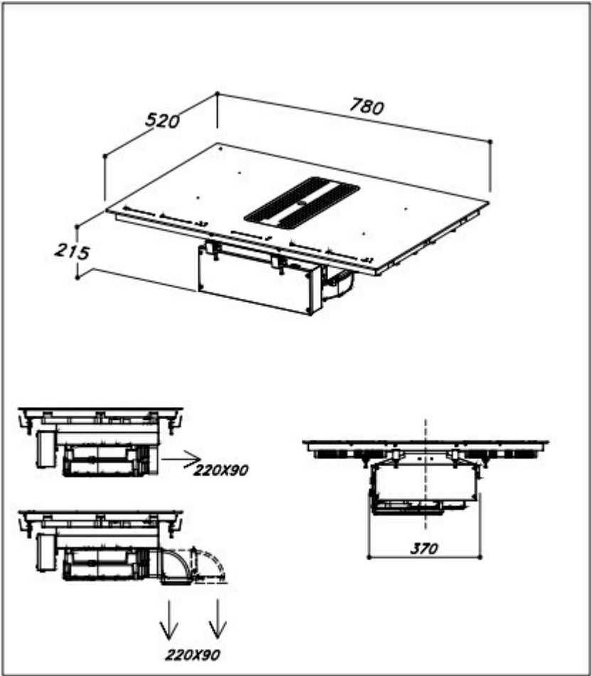
Apertura Top: 750mm X 490mm Rectangular opening: 750mm X 490mm
