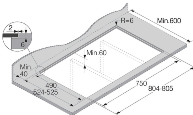
Flush built
