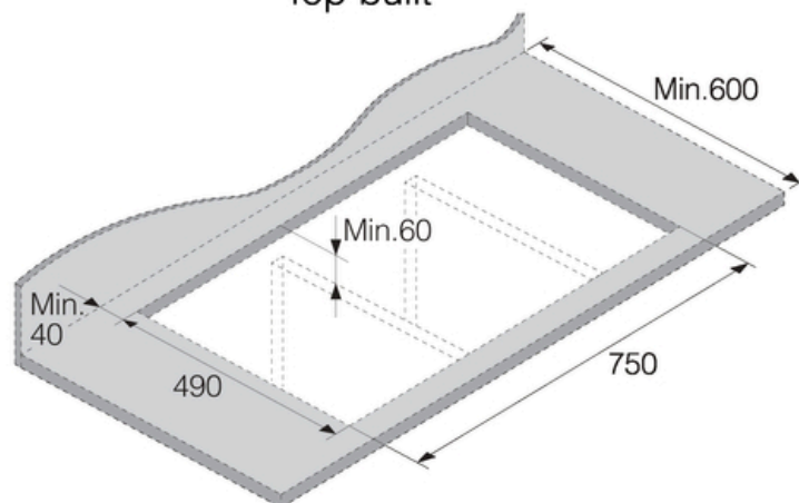
Top built
