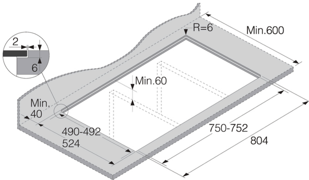
Flush-built
