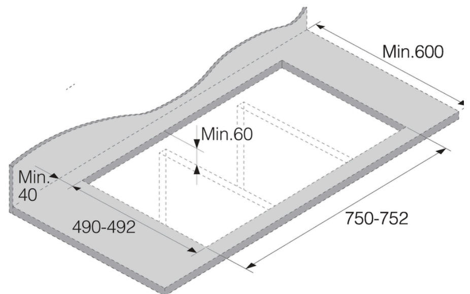
Top-built
